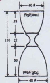
Shape & Nominal Dimensions of Combined Liquor Measures 60 ml. & 30 ml.
